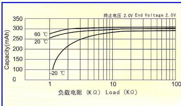
Load-capacity
